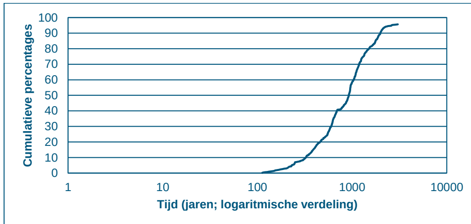
Figuur 4-3 Responsecurve Holtien (Royal Haskoning, 2008)
