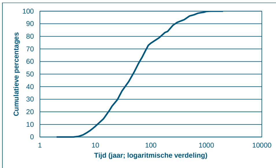
Figuur 4-4 Responsecurve Gasselte (Royal Haskoning, 2003)
