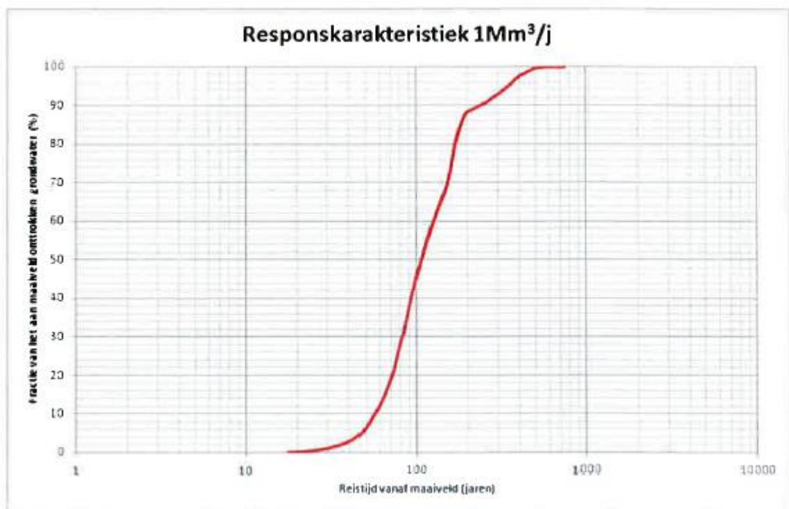
Figuur 4-4 Responsecurve Assen-west (Sweco, 2015)
