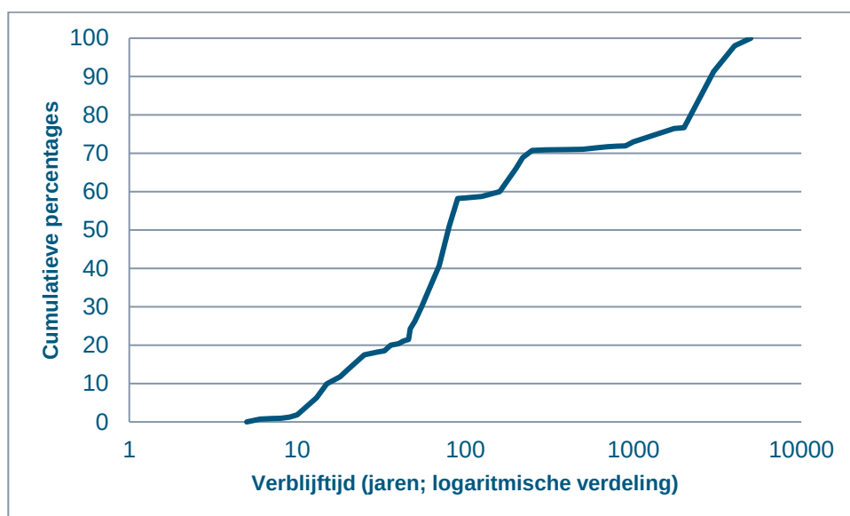
Figuur 4-4 Responsecurve Beilen (Adviesbureau Harry Boukes, 1996)
