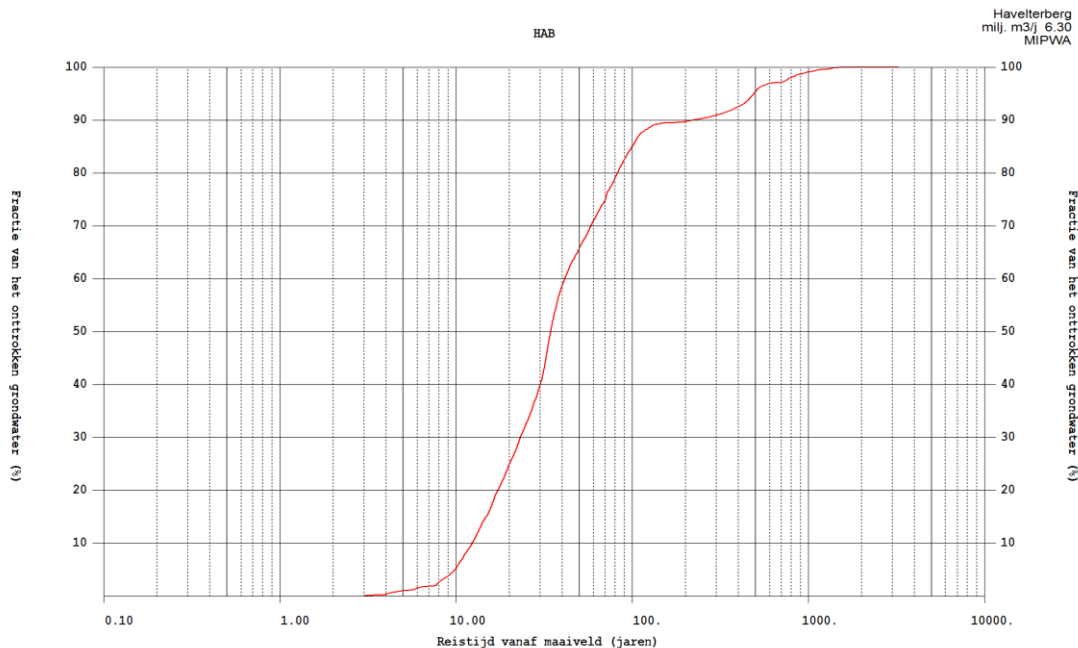
Figuur 4-4 Responsecurve Havelterberg (Vitens, 2003)
